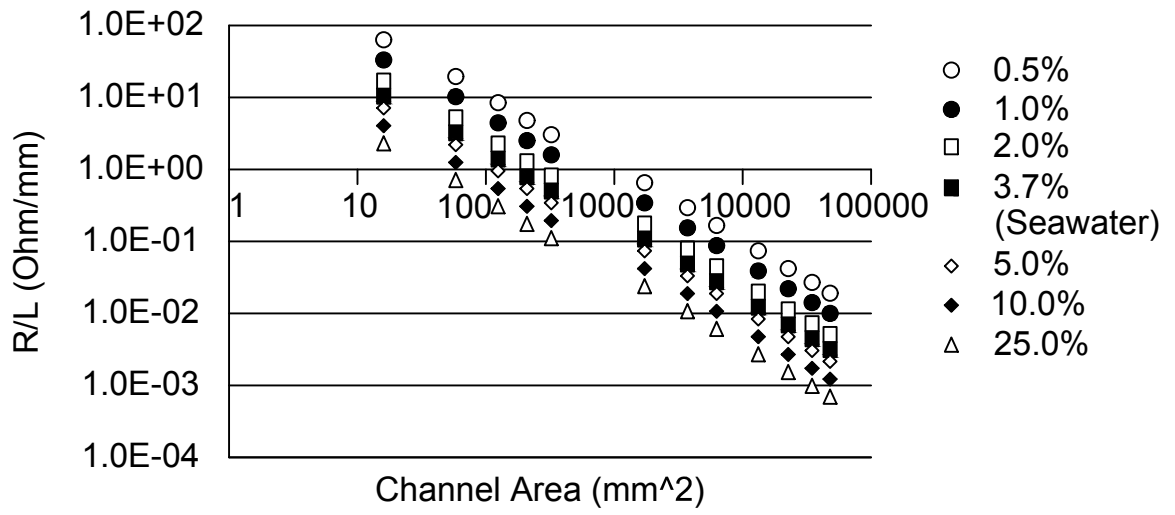
Resistance vs Area, per 1mm length
